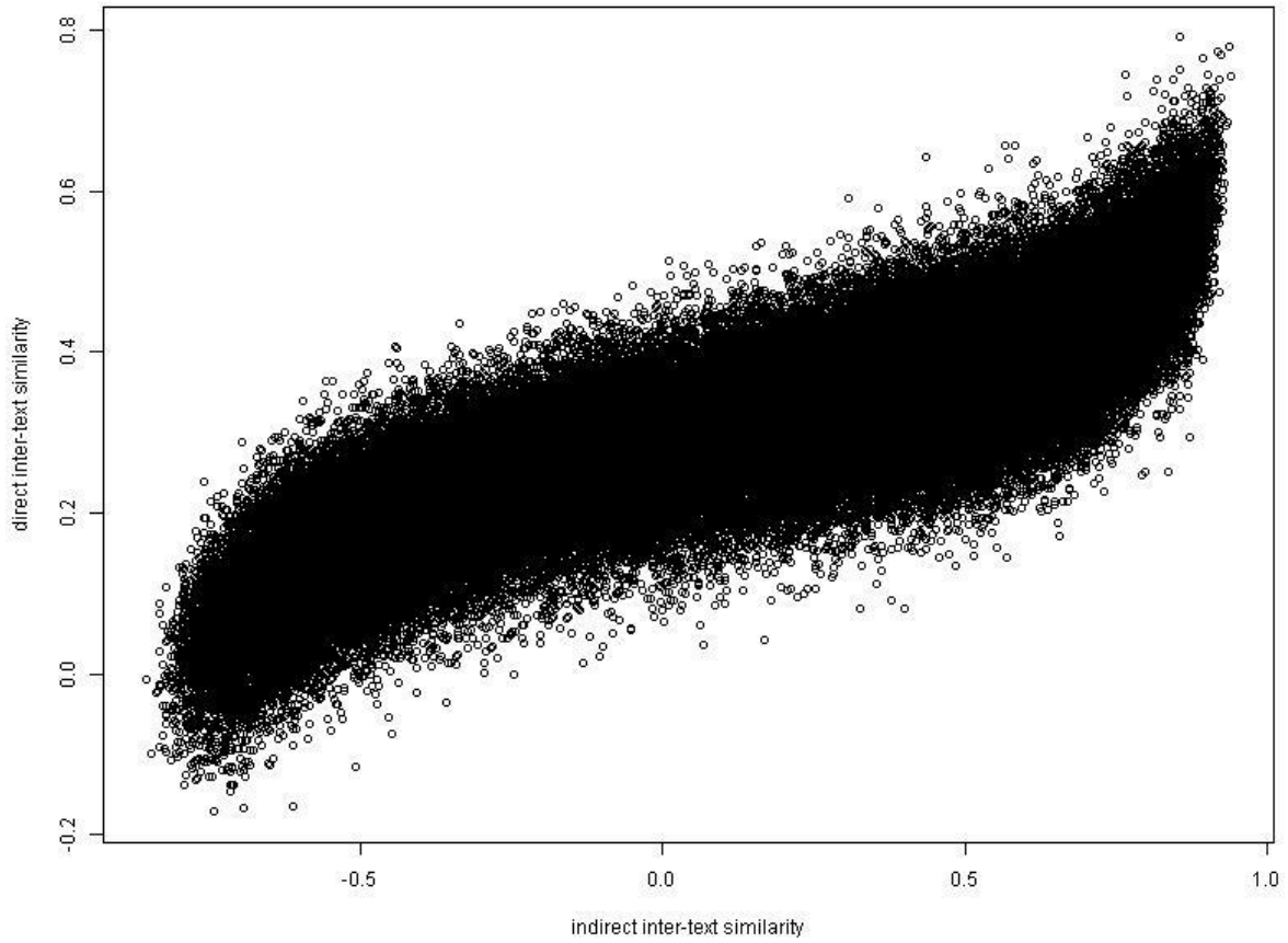
Figure 4. Comparison of direct and indirect inter-text similarities: LOB versus Pentaglossal Corpus (2/3-grams, fr+itet).
