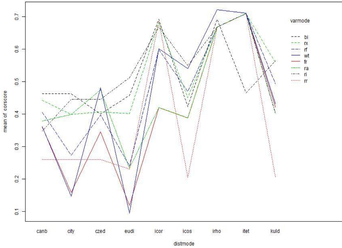
Correlation with criterion by distance & variable modes (1/1-,2/3-grams).
