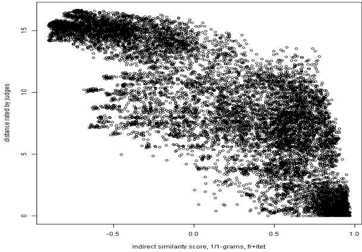
DE/EN anchor-based similarity test, 5gcorpus ( r = -0.8334 ).
